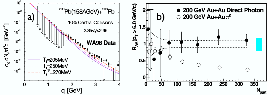
Fig. 3. a) WA98 results described by QGP effects and pQCD; b) PHENIX yields for \gamma and \pi^0 at p_t > 6 GeV vs. the number of participating nucleons, scaled from AuAu to NN.
